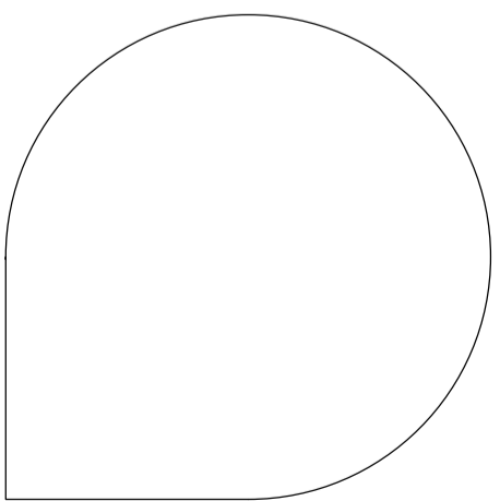
Boy's Surface - a paper cutout model designed by Chris Hilder ( http://teach.hilderbuild.com/tiki-index.php?page=Paper Boy's ) based on a design by Joe Fields ( http://www.southernct.edu/~fields/topology/Boys_surface.html )
