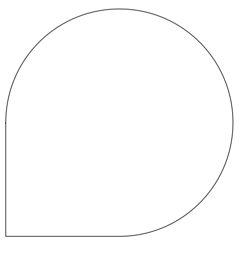
Boy's Surface - a paper cutout model designed by Chris Hilder ( http://teach.hilderbuild.com/tiki-index.php?page=Paper Boy's ) based on a design by Joe Fields ( http://www.southernct.edu/~fields/topology/Boys_surface.html )
